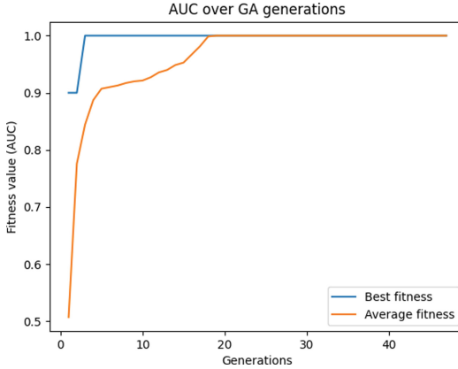
Fig. 5. Fitness value evaluation over GA generations.
