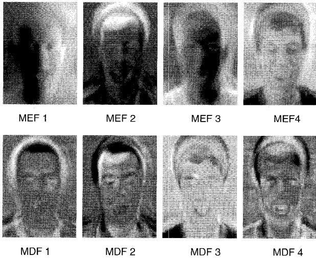
Fig. 2. A sample of MEF and MDF vectors treated as images. The MEF vectors show the tendency of the principal components to capture major variations in the training set, such as lighting direction. The MDF vectors show the ability of the MDFs to discount those factors unrelated to classification. The training images used to produce these vectors are courtesy of the Weizmann Institute.
