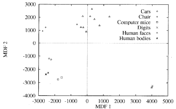
(b) MDF space
