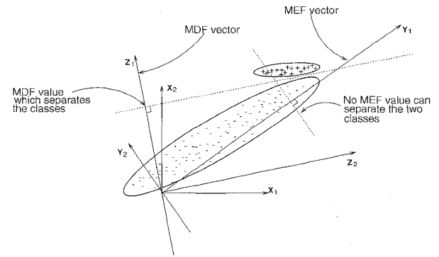
Fig. 1. Problems with the MEF projection for class separation.
