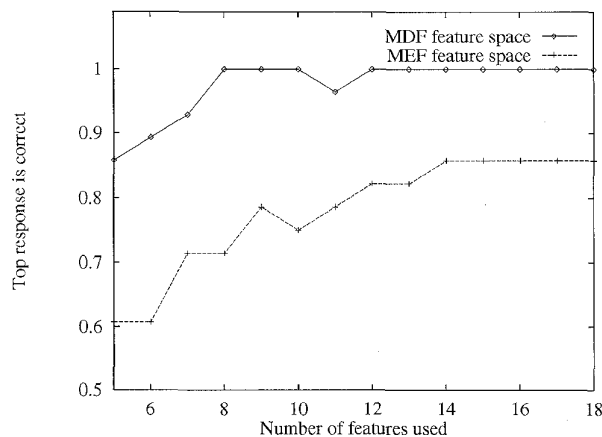
Fig. 4. The performance of the system for different numbers of MEF and MDF features, respectively. The number of features from the subspace used was varied to show how the MDF subspace outperforms the MEF subspace. 95% of the variance for the MDF subspace was attained when 15 features were used; 95% of variance for the MEF subspace did not occur until 37 features were used. Using 95% of the MEF variance resulted in an 89% recognition rate, and that rate was not improved using more features.
