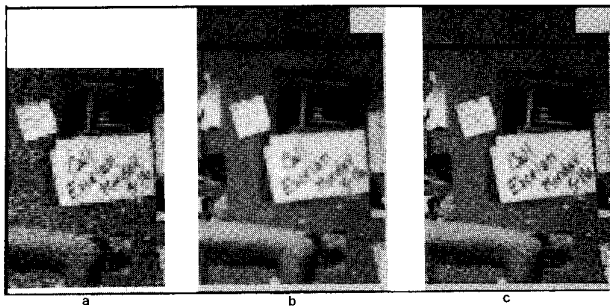
FIG. 6. Superresolution from ten 50 \times 70 noisy monochrome images. (a) One of the 10 low-resolution images. (b) The initial guess: average of the low-resolution images after registration. (c) Improved resolution image.
