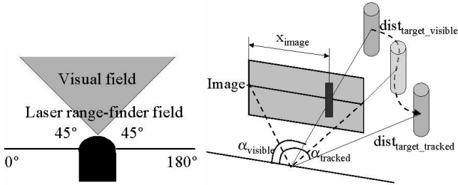
(a) Space coverage using laser rangefinder and camera (b) Principle for target tracking by merging vision and laser data Fig. 4. Merging laser and visual information for tracking
