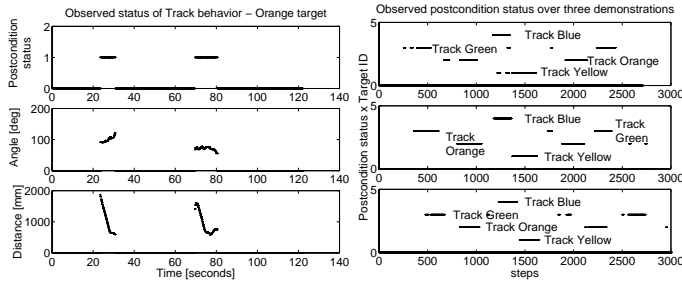
(a) Observed values of a Track behavior's parameters and the status of its postconditions (b) Observed status of all the behaviors' postconditions during three different demonstrations
