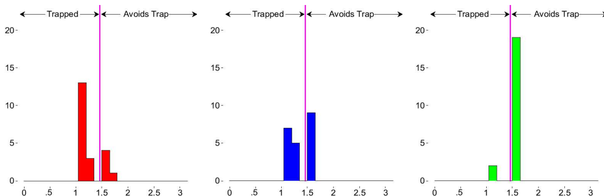
Figure 2: Distribution of RC values. Left: GA alone. Middle: With case injection. Right: Case Injection and fitness biasing.
