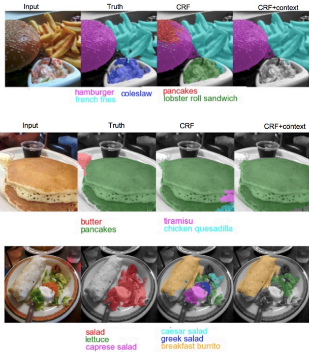
Figure 5. Examples of semantic image segmentation on some images from the Food201-Segmented test set. First column: original image. Second column: ground truth. Third column: predictions using CNN/CRF. Fourth column: predictions using CNN/CRF with multilabel context. Best viewed in color.
