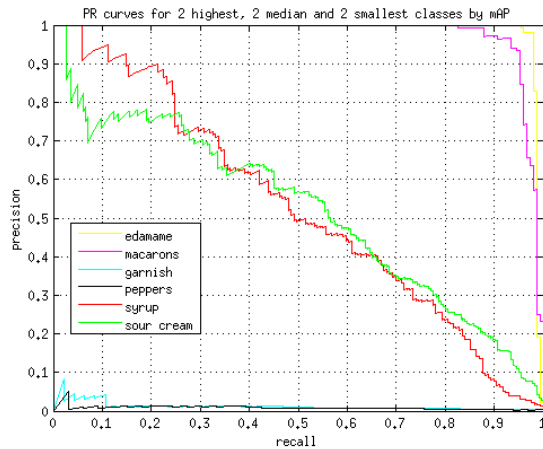
Figure 4. Precision-recall curves for 6 classes, ranging from best to worst, on the Food201-MultiLabel dataset.
