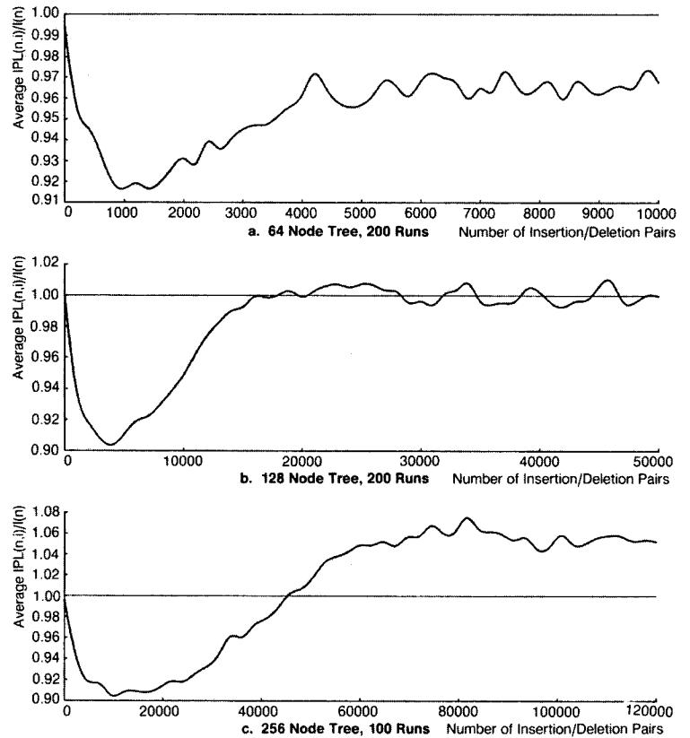
FIGURE 5. Asymmetric Deletions.
