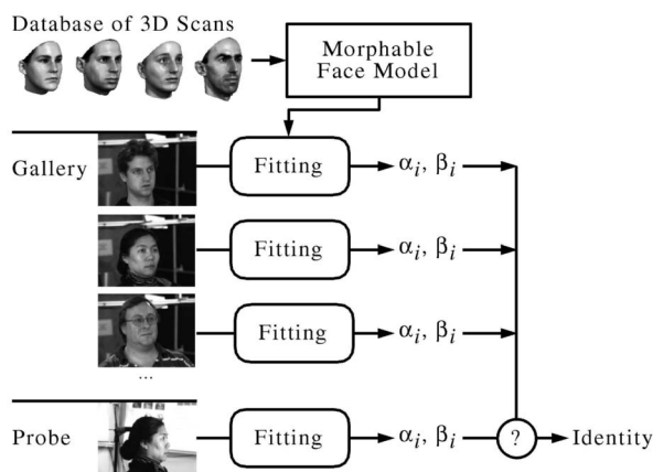
Fig. 1. Derived from a database of laser scans, the 3D morphable face model is used to encode gallery and probe images. For identification, the model coefficients \alpha_i, \beta_i of the probe image are compared with the stored coefficients of all gallery images.
