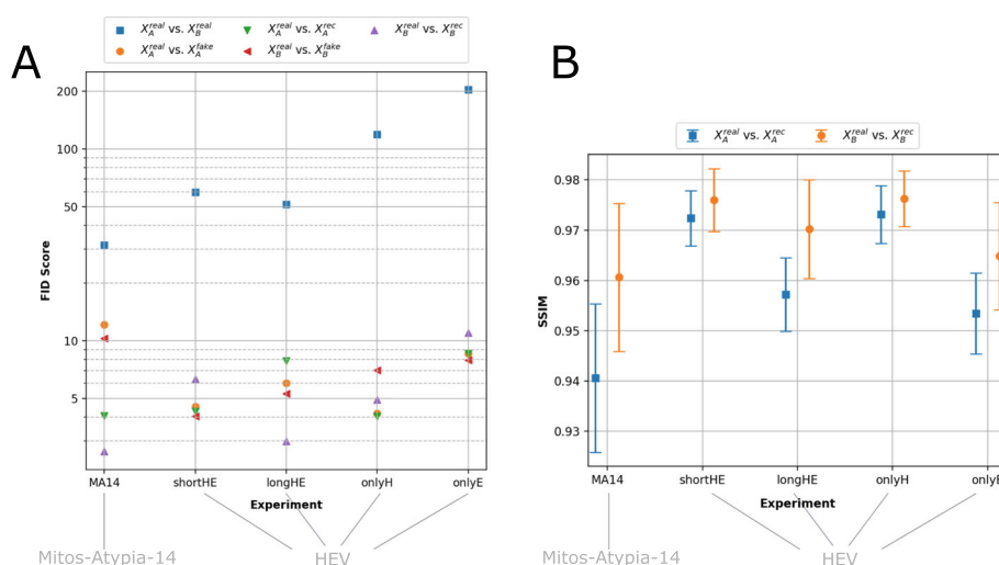
Fig. 5 Evaluation of our experiments using FID and SSIM scores.
