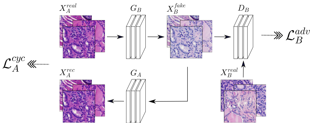
Fig. 1 Illustration of the applied CycleGAN architecture for mapping images from domain A to domain B.
