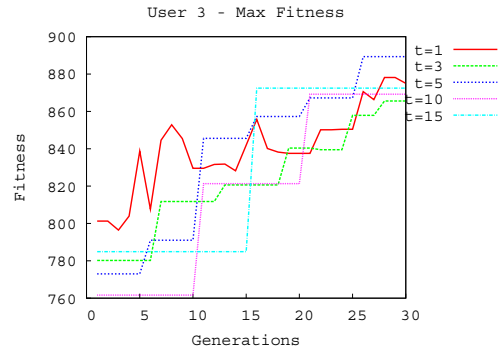
Fig. 5. Fitness performance of user 3. The plot shows the best individuals in the population.
