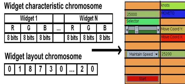
Fig. 2. UI encoding consists of two chromosomes. The widget characteristic chromosome encodes the color of each widget in a bit format. The widget layout chromosome encodes the position of the widgets in the grid. Widgets are identified by integer IDs greater than 0 and empty cells in the grid are identified with 0s.
