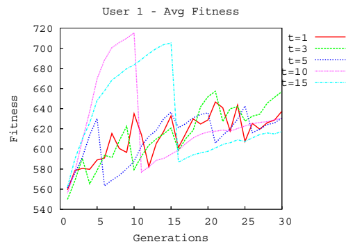
Fig. 6. Fitness performance of user 1. The plot shows the average individuals in the population.
