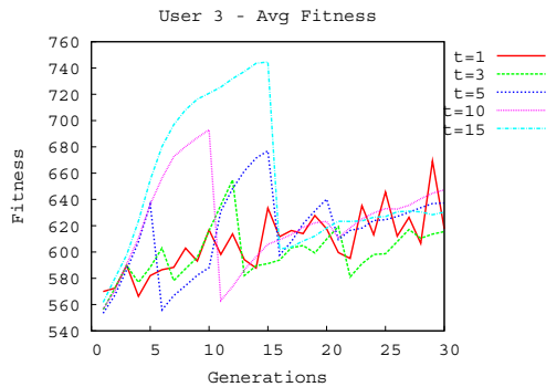
Fig. 8. Fitness performance of user 3. The plot shows the average individuals in the population.
