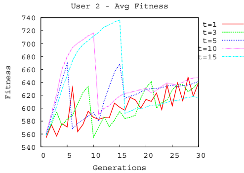
Fig. 7. Fitness performance of user 2. The plot shows the average individuals in the population.
