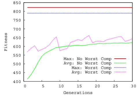
Fig. 9. Fitness performance of population with comparison to user selected worst turned off and comparison to the user selected best turned on.
