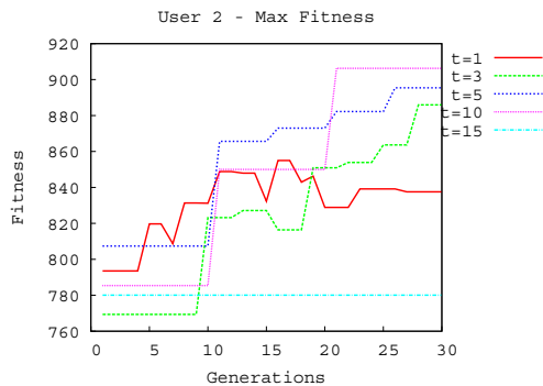
Fig. 4. Fitness performance of user 2. The plot shows the best individuals in the population.
