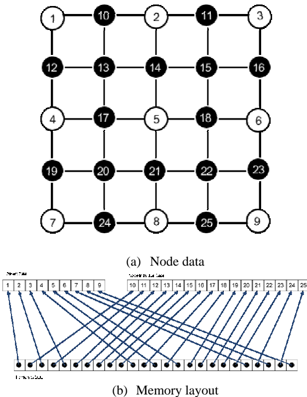
Figure 3: Node data shown in (a) represents the memory layout shown in (b)
