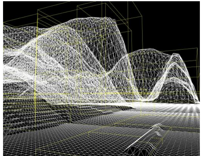
Figure 4: A quadtree displaying the bounding boxes of each node. Bounding boxes are culled against the viewing frustum to quickly eliminate nodes during refinement
