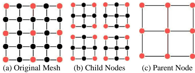
Figure 2: The simplification process to create a quadtree. The original mesh (a) is separated into m \times m nodes ( m=5 ) (b) where each 2 \times 2 block creates a parent node (c)
