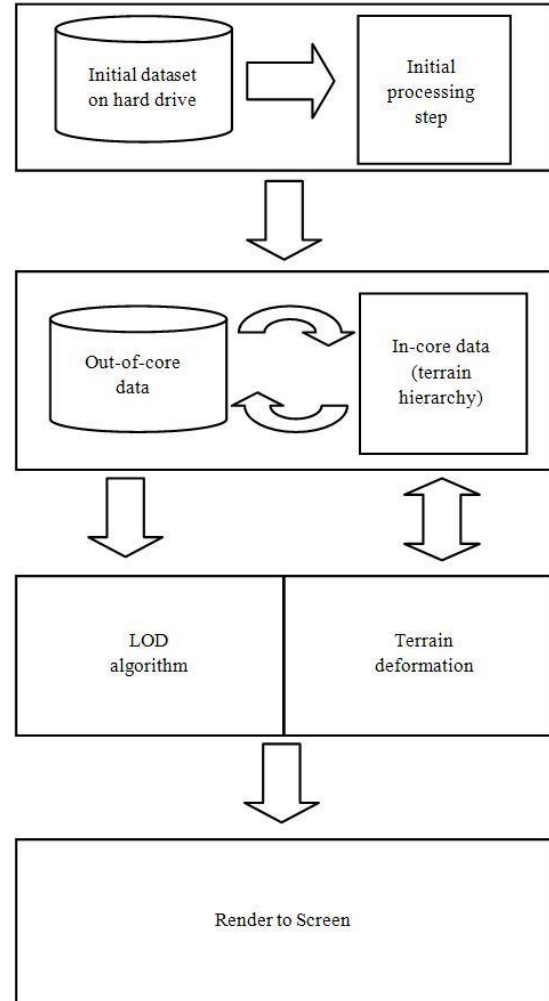
Figure 1: Block diagram showing the flow of the data through the system
