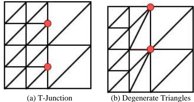
Figure 5: T-Junctions appear at the neighboring nodes of different levels of detail. Omitting vertices via degenerate triangles removes any possible cracks from the mesh
