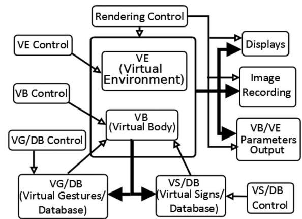
Fig. 1. sEditor architecture (VE: Virtual Environment; VB: Virtual Body; VG: Virtual Gestures; VS: Virtual Signs; DB: Database).
