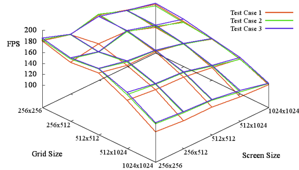
Fig. 8. Total FPS for all three cases.
