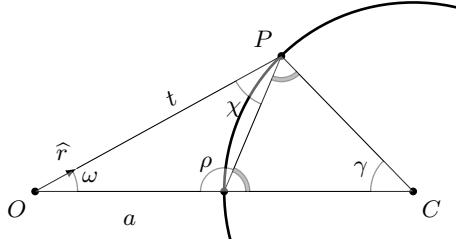
Fig. 2. The intersection position in eye space.
