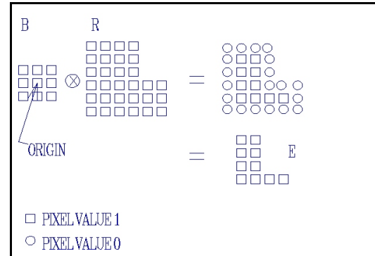
Figure 5.10. Erosion of R by B.
