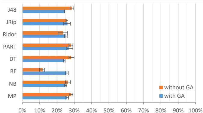
Fig. 7. SSL Performance
