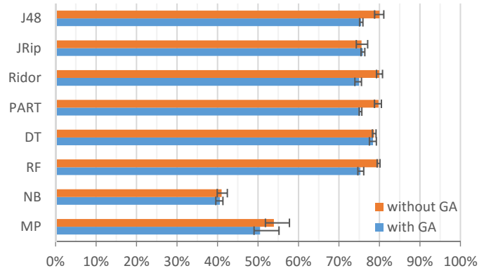
Fig. 4. UDP Performance
