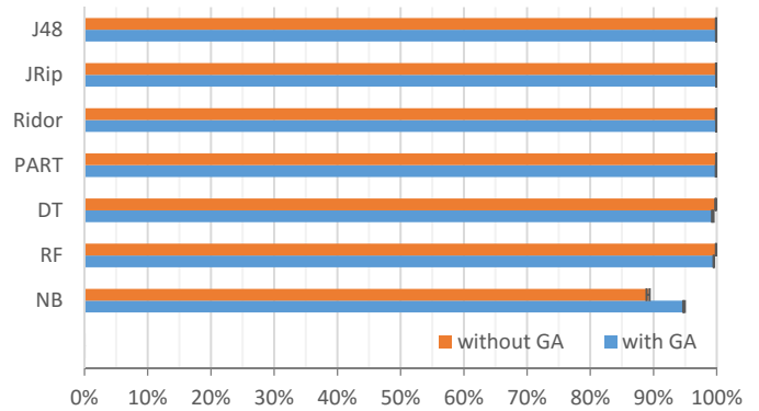
Fig. 3. TCP Performance
