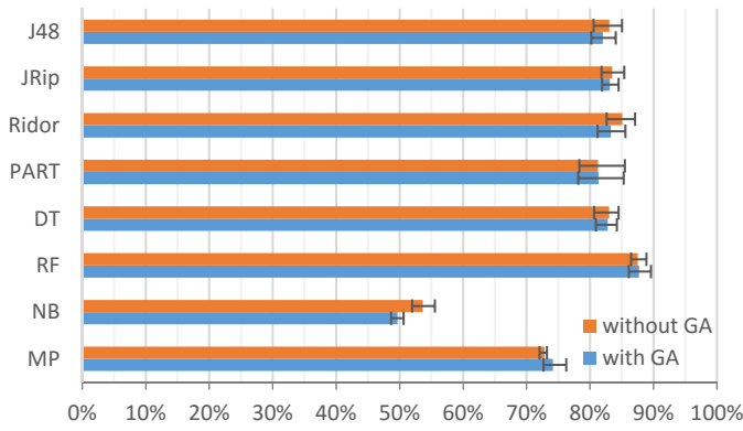
Fig. 5. HTTP Performance
