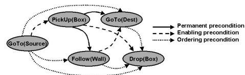
Figure 2: Example of a behavior network
