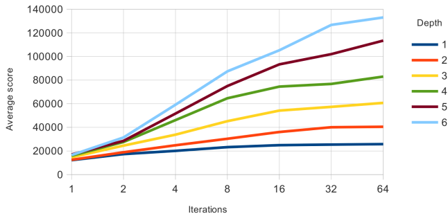
Figure 2: ADLS Results.
